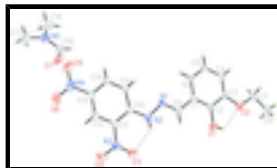
Fig. 1. : the molecular structure of (I) with displacement ellipsoids drawn at the 30% probability level. Intramolecular hydrogen bonds are shown as dashed lines.
